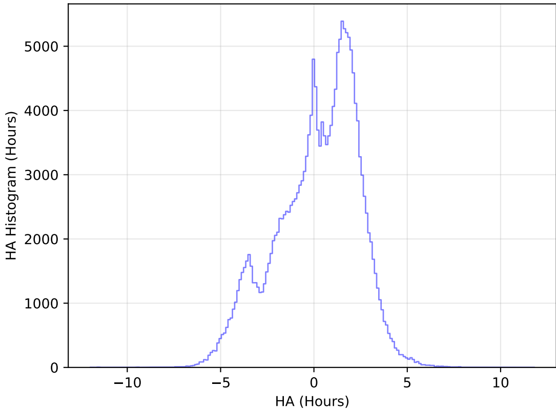
ddf_acor_sf10_lsf40_lsr10_v3.4_10yrs All sky g band: HA Histogram
