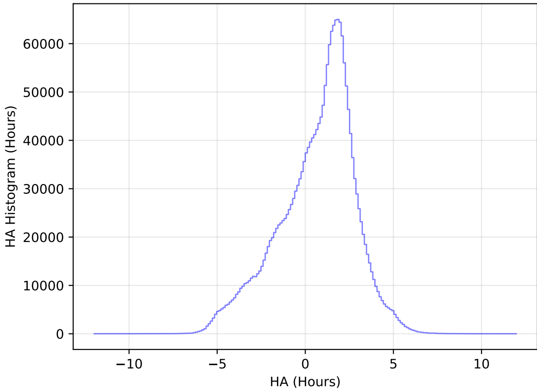
ddf_acor_sf10_lsf40_lsr10_v3.4_10yrs All sky all bands: HA Histogram
