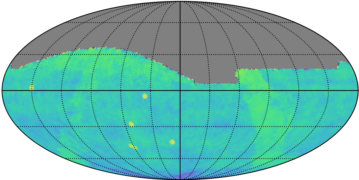
ddf_acor_sf10_lsf40_lsr10_v3.4_10yrs gri All sky: Fraction of visits in pairs (10-60 min)
