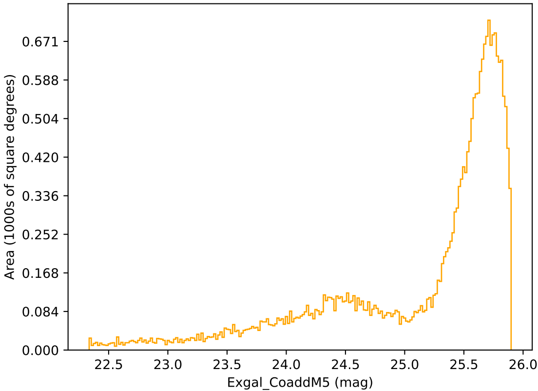
ddf_acor_sf10_lsf40_lsr10_v3.4_10yrs Yr 1 r band: Exgal_CoaddM5
