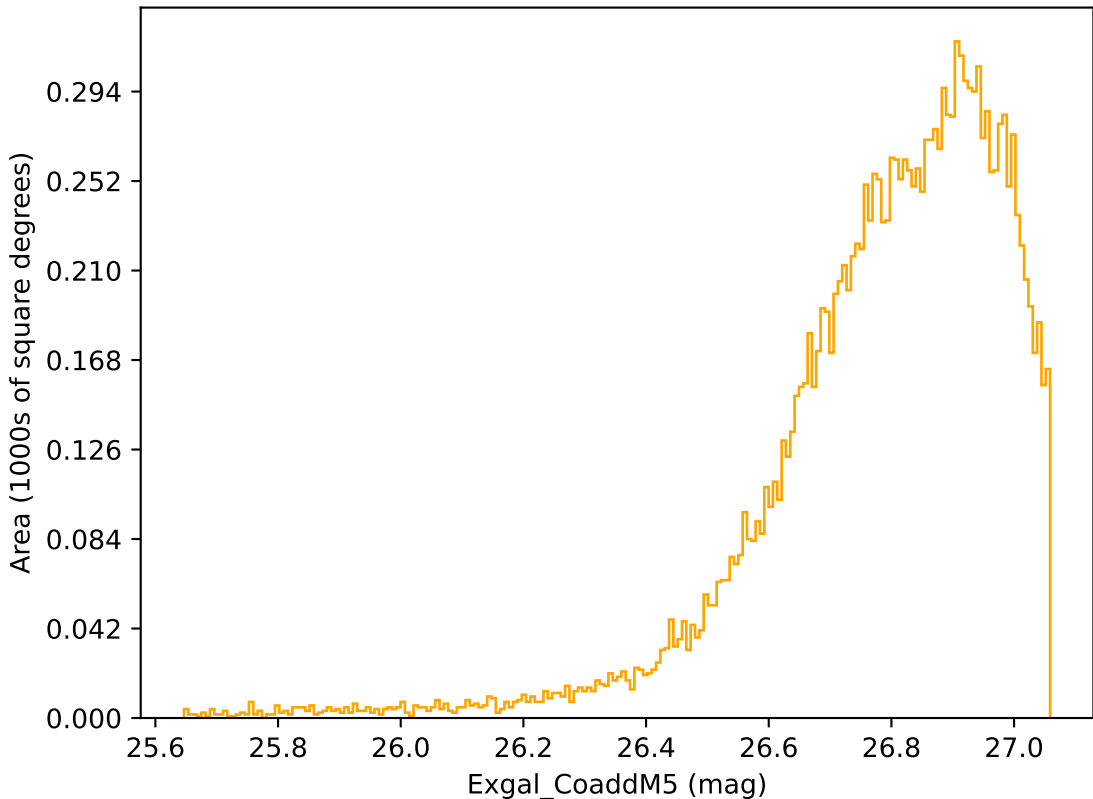
ddf_acor_sf10_lsf40_lsr10_v3.4_10yrs WFD r band: Exgal_CoaddM5
