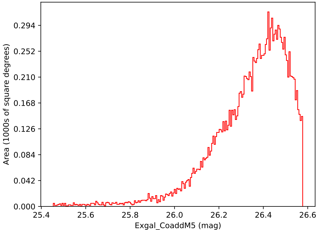
ddf_acor_sf10_lsf40_lsr10_v3.4_10yrs WFD i band: Exgal_CoaddM5
