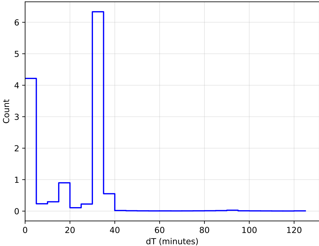
ddf_acor_sf10_lsf40_lsr10_v3.4_10yrs All sky: DeltaT Histogram
