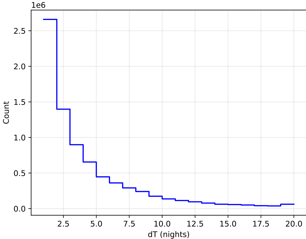
ddf_acor_sf10_lsf40_lsr10_v3.4_10yrs WFD all bands: DeltaNight Histogram
