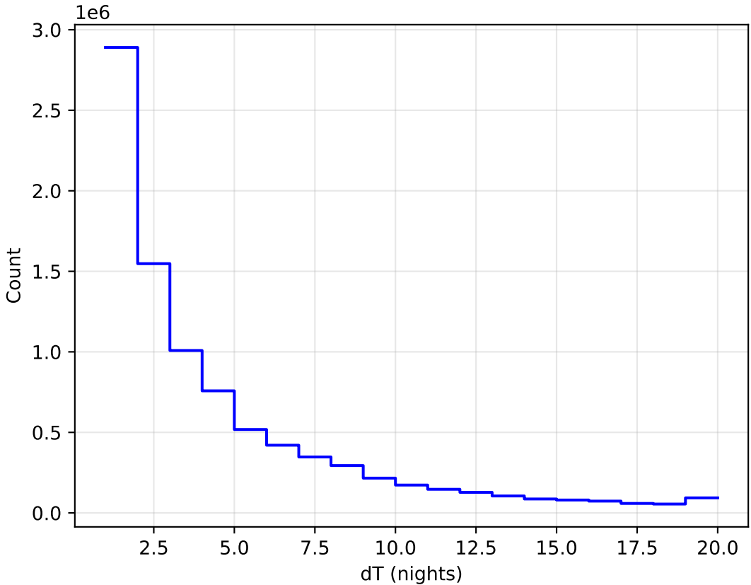
ddf_acor_sf10_lsf40_lsr10_v3.4_10yrs All sky all bands: DeltaNight Histogram
