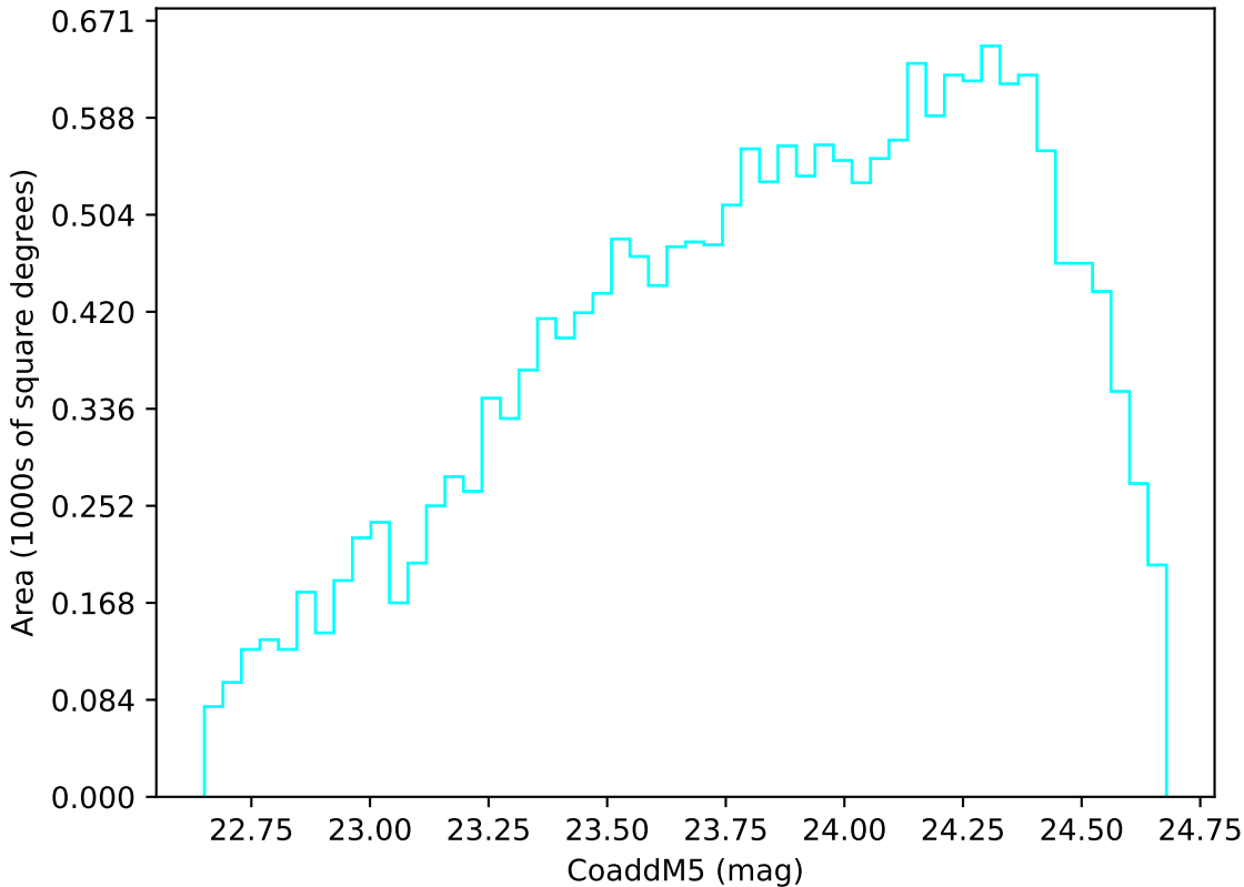
ddf_acor_sf10_lsf40_lsr10_v3.4_10yrs Yr 3-4 u band: CoaddM5
