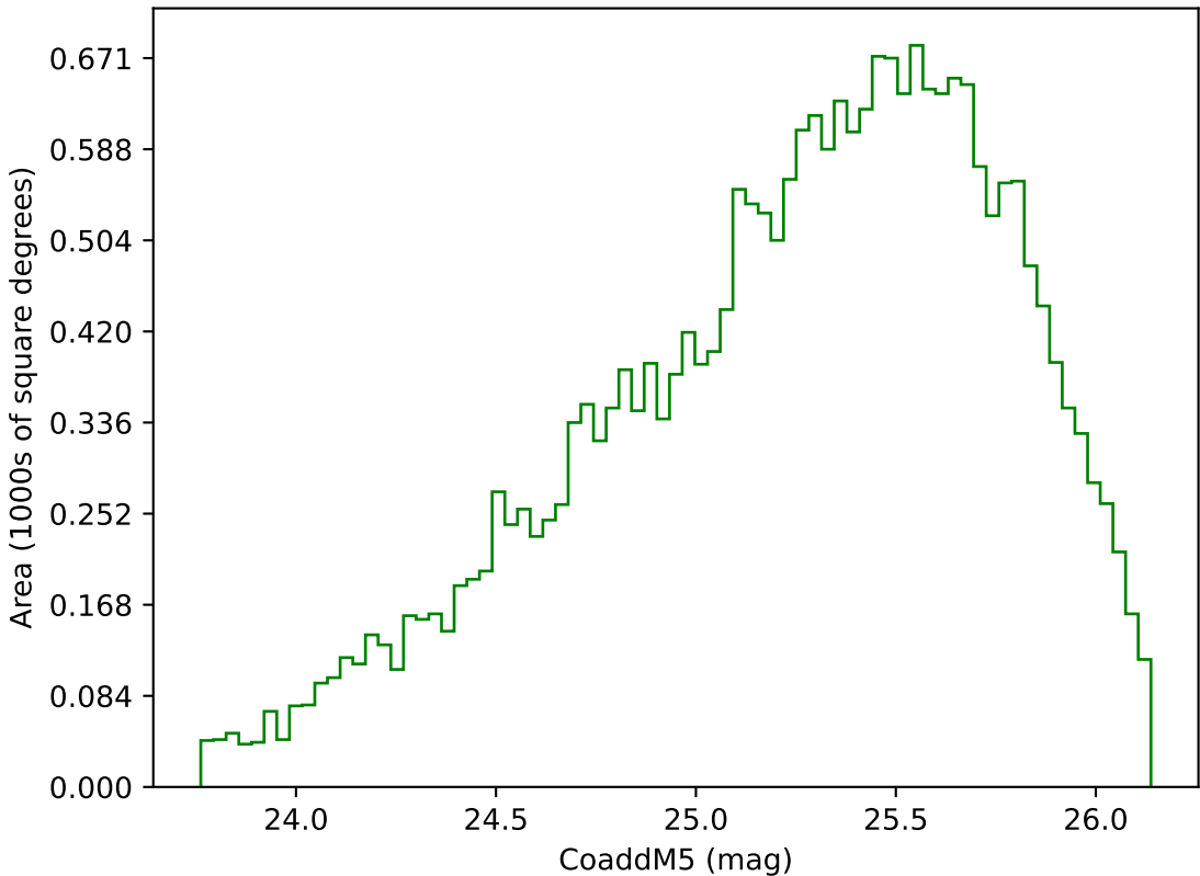
ddf_acor_sf10_lsf40_lsr10_v3.4_10yrs Yr 3-4 g band: CoaddM5
