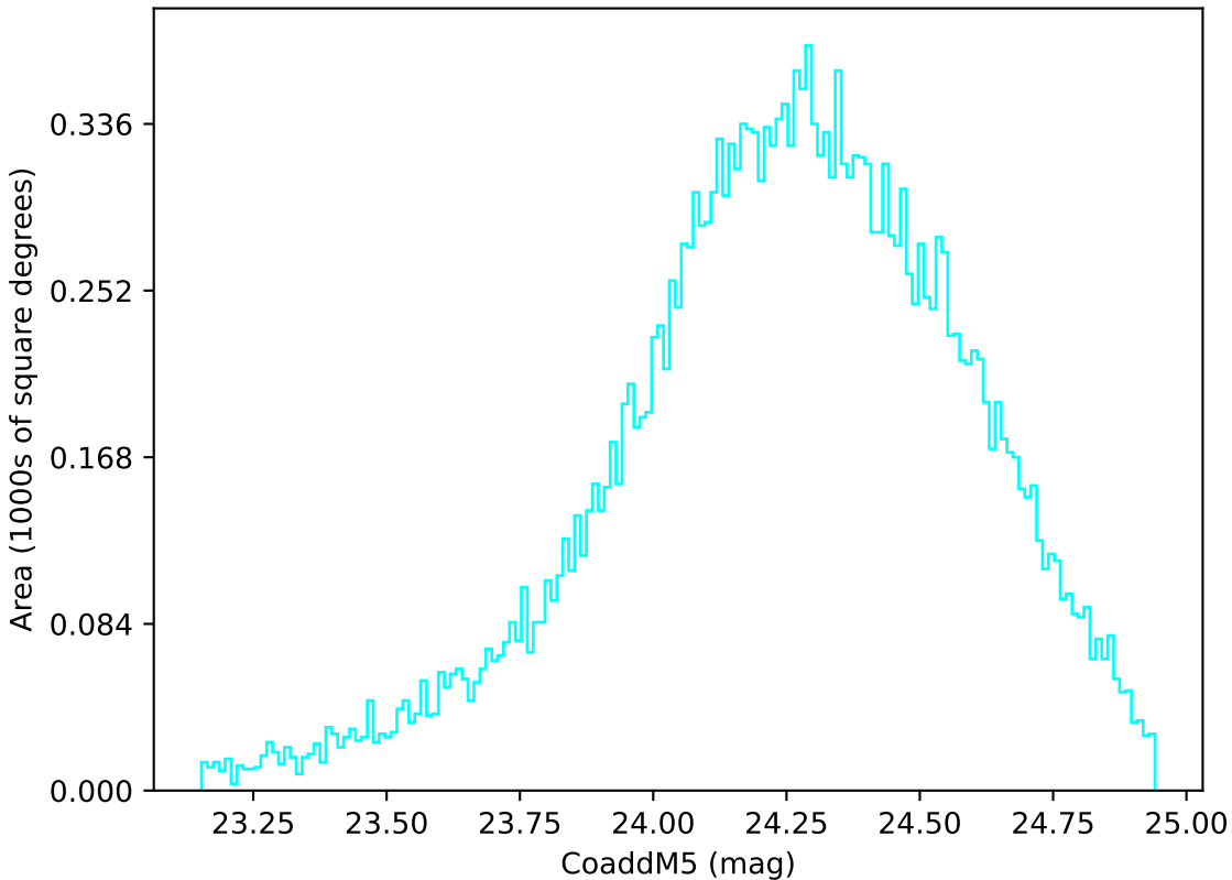
ddf_acor_sf10_lsf40_lsr10_v3.4_10yrs Yr 1 u band: CoaddM5
