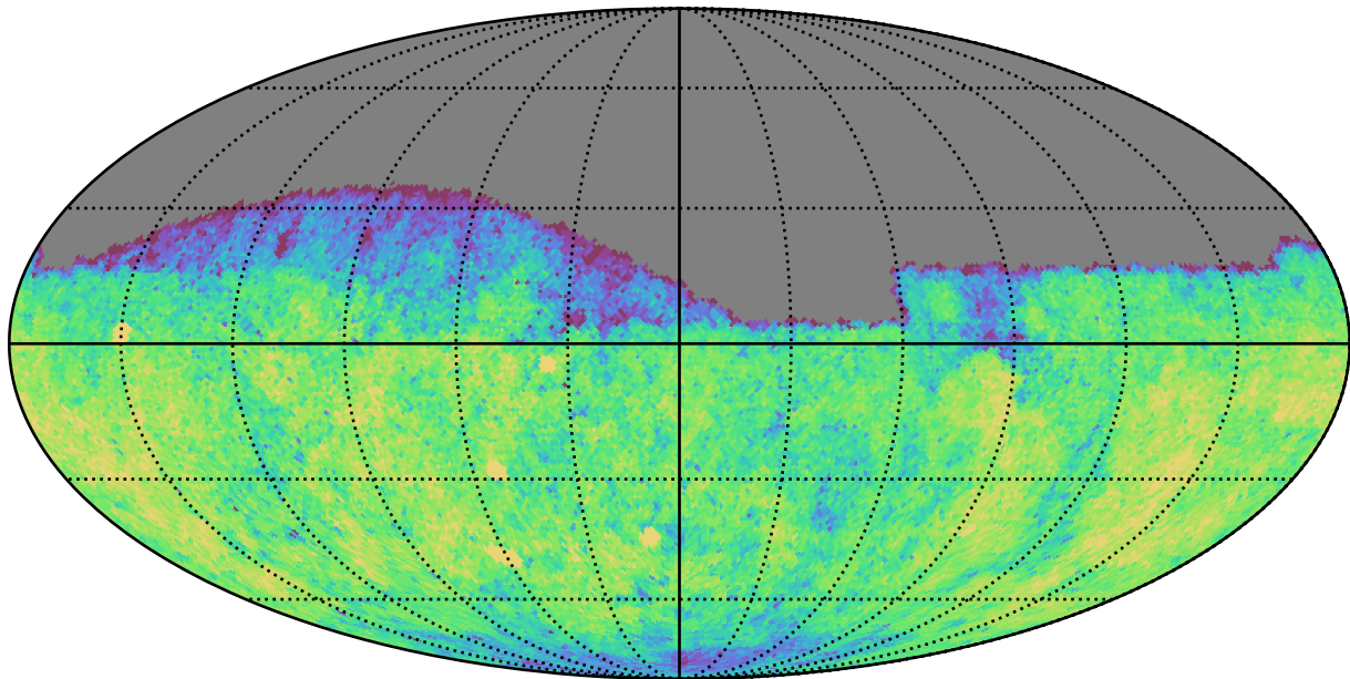
ddf_acor_sf10_lsf40_lsr10_v3.4_10yrs Yr 1 g band: CoaddM5
