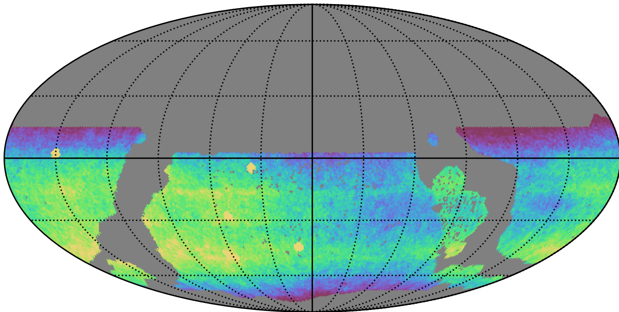
ddf_acor_sf10_lsf40_lsr10_v3.4_10yrs WFD r band: CoaddM5
