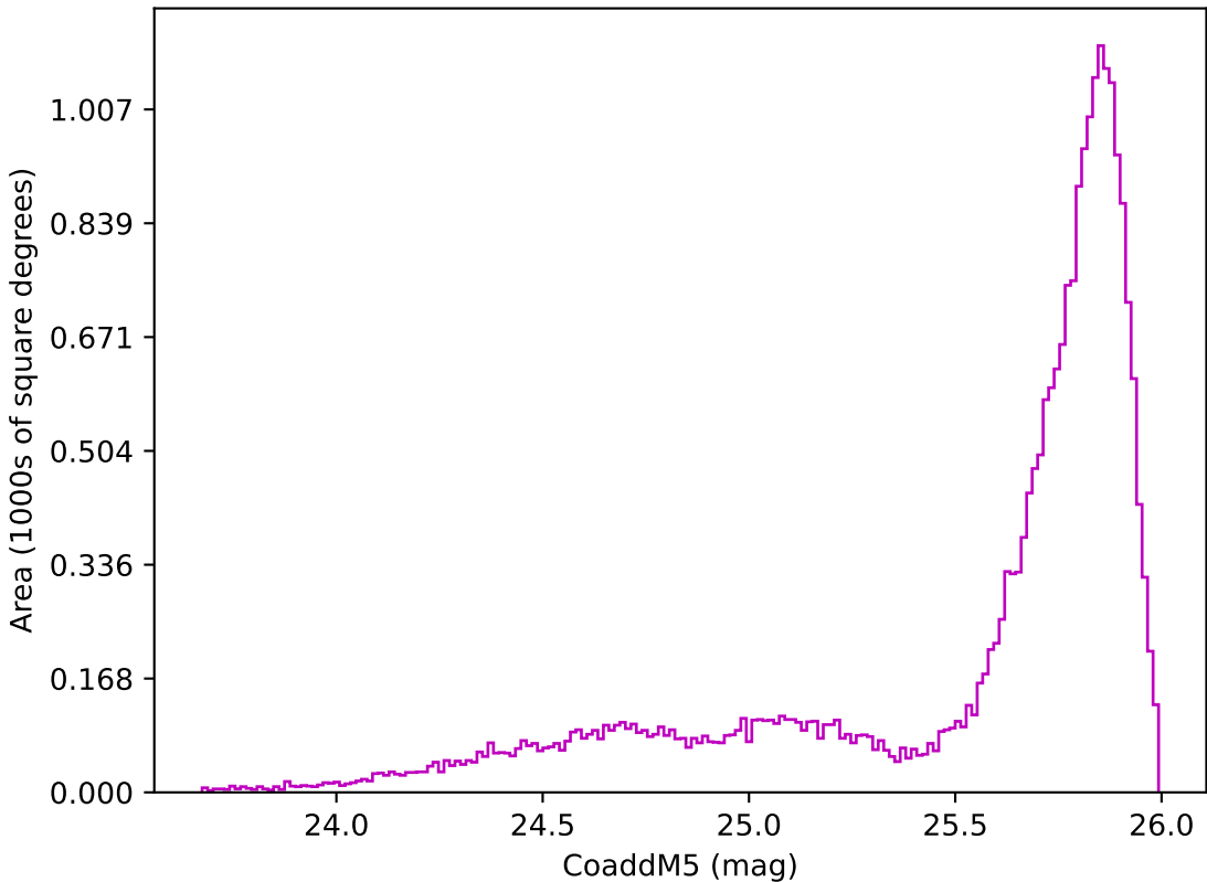
ddf_acor_sf10_lsf40_lsr10_v3.4_10yrs All sky z band: CoaddM5
