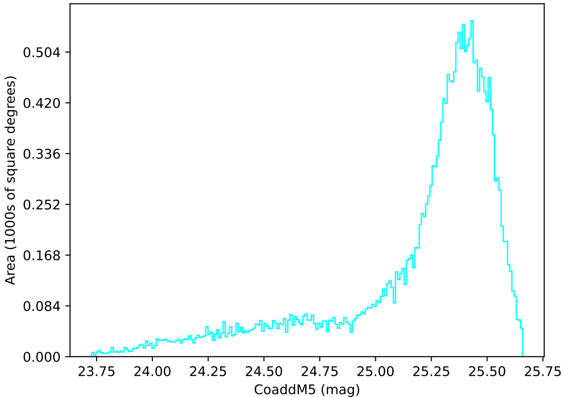
ddf_acor_sf10_lsf40_lsr10_v3.4_10yrs All sky u band: CoaddM5
