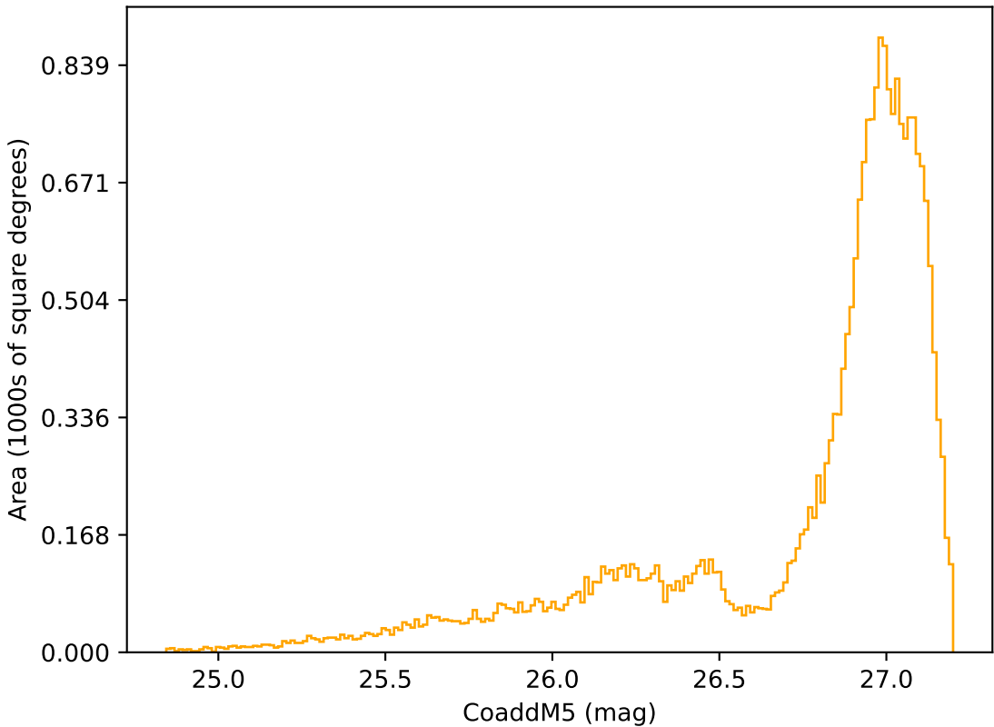
ddf_acor_sf10_lsf40_lsr10_v3.4_10yrs All sky r band: CoaddM5
