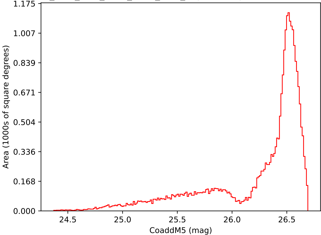
ddf_acor_sf10_lsf40_lsr10_v3.4_10yrs All sky i band: CoaddM5
