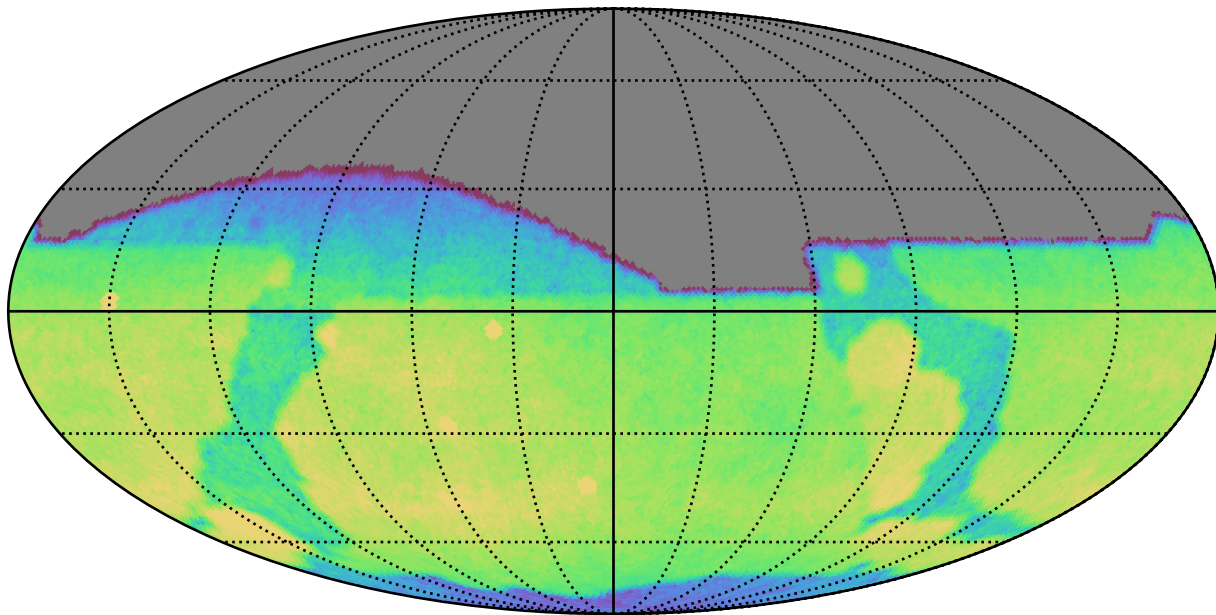
ddf_acor_sf10_lsf40_lsr10_v3.4_10yrs All sky g band: CoaddM5
