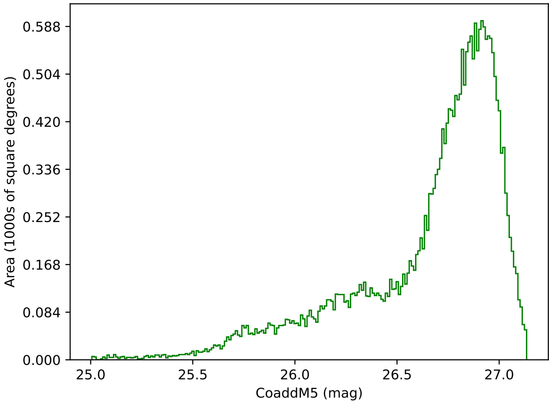
ddf_acor_sf10_lsf40_lsr10_v3.4_10yrs All sky g band: CoaddM5
