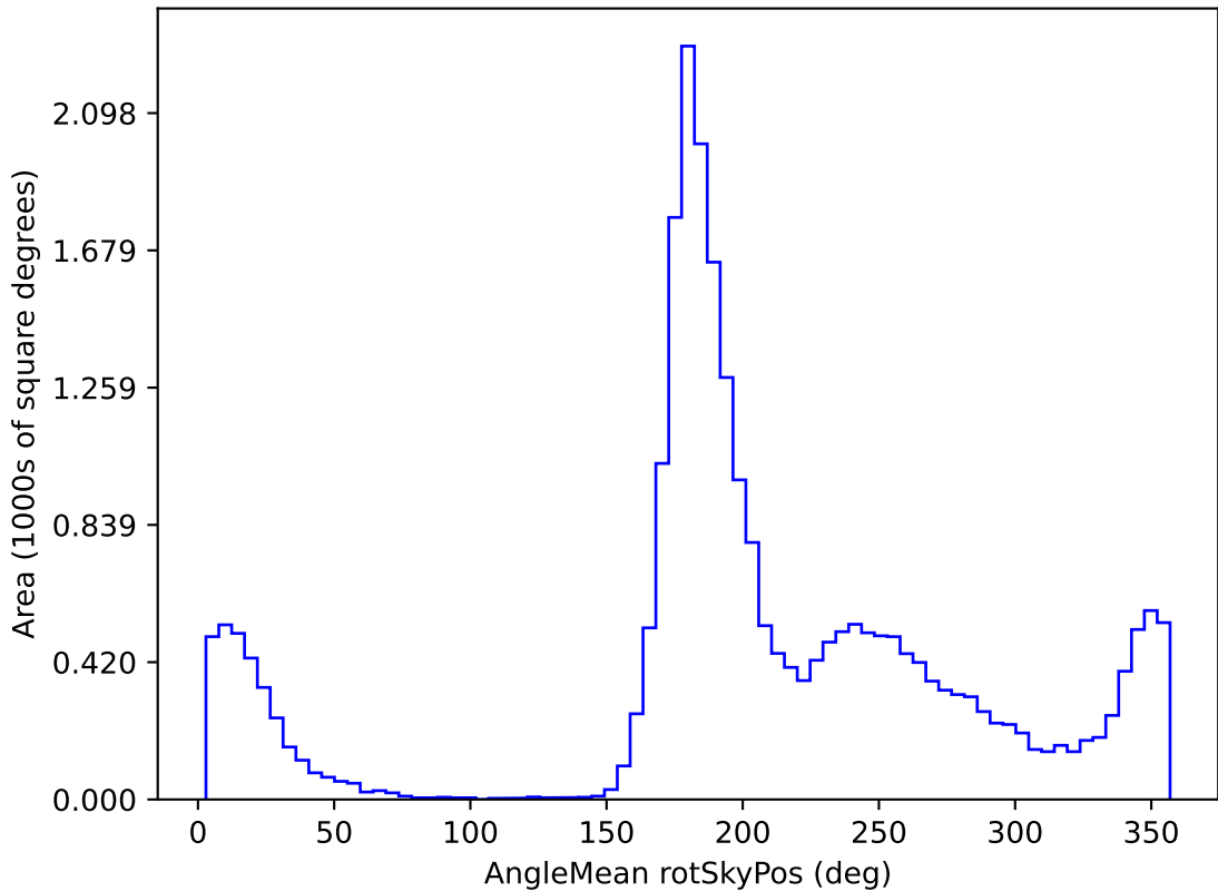
ddf_acor_sf10_lsf40_lsr10_v3.4_10yrs All sky i band: AngleMean rotSkyPos
