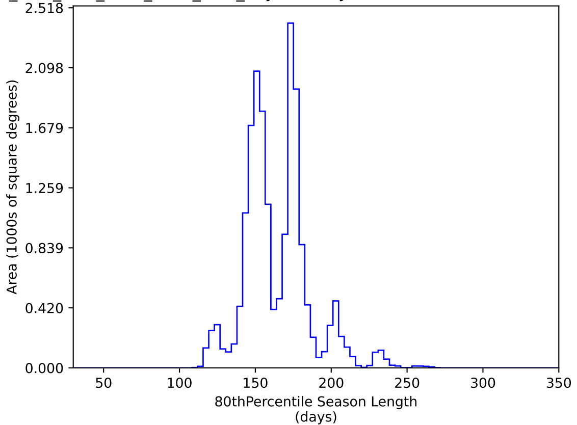
ddf_acor_sf10_lsf40_lsr10_v3.4_10yrs WFD y band: 80thPercentile Season Length
