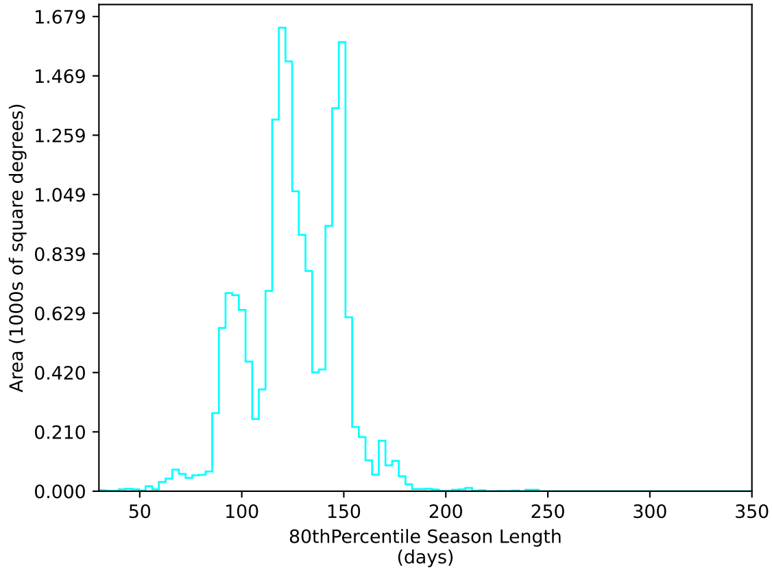
ddf_acor_sf10_lsf40_lsr10_v3.4_10yrs WFD u band: 80thPercentile Season Length
