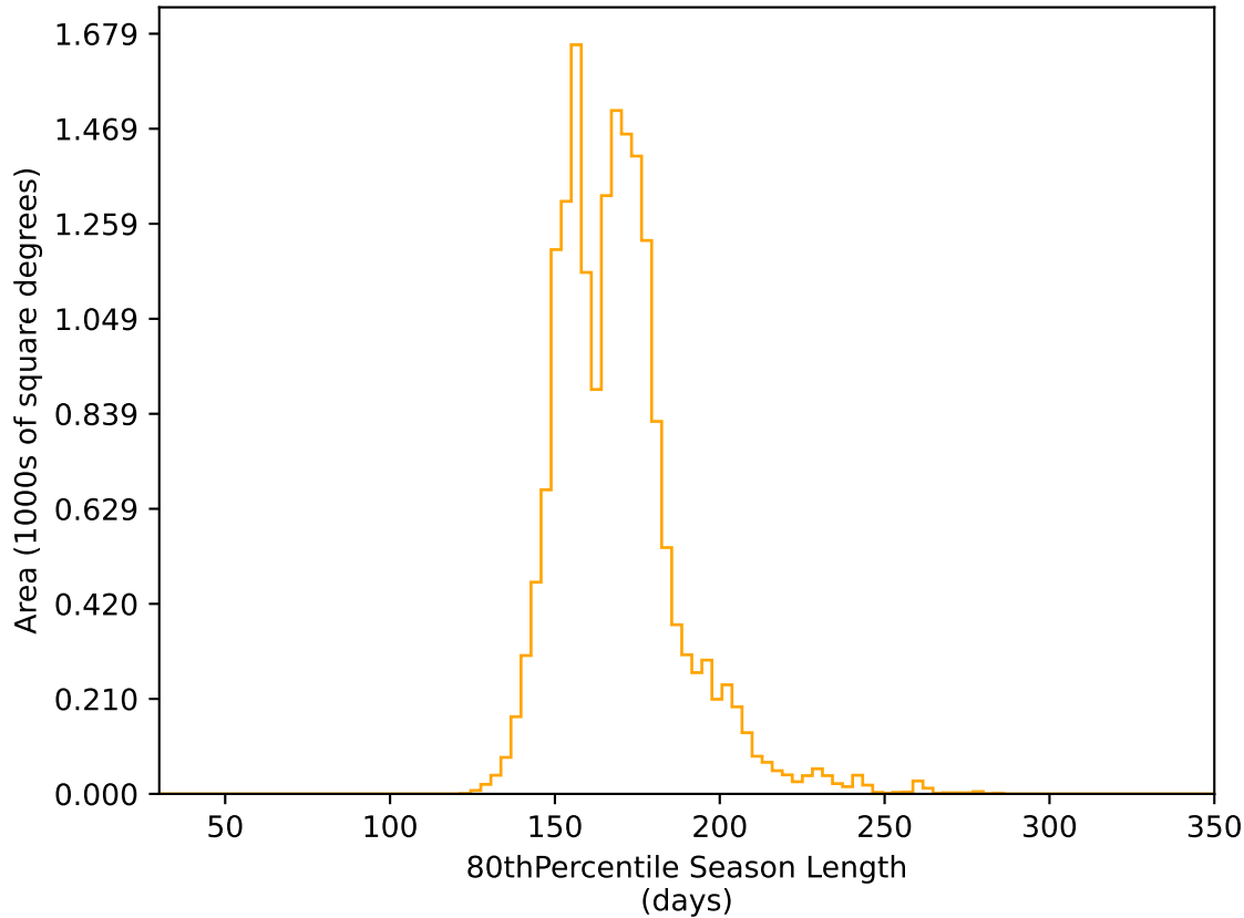
ddf_acor_sf10_lsf40_lsr10_v3.4_10yrs WFD r band: 80thPercentile Season Length
