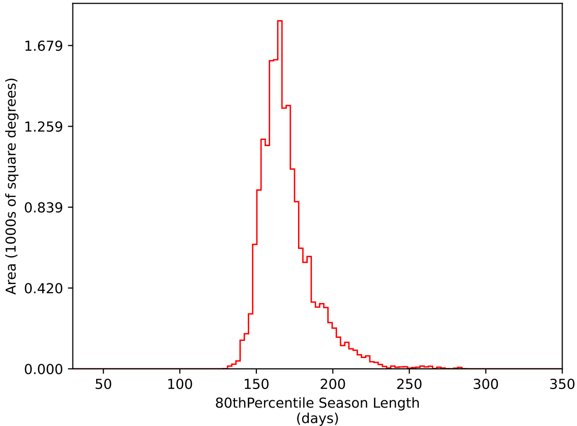
ddf_acor_sf10_lsf40_lsr10_v3.4_10yrs WFD i band: 80thPercentile Season Length
