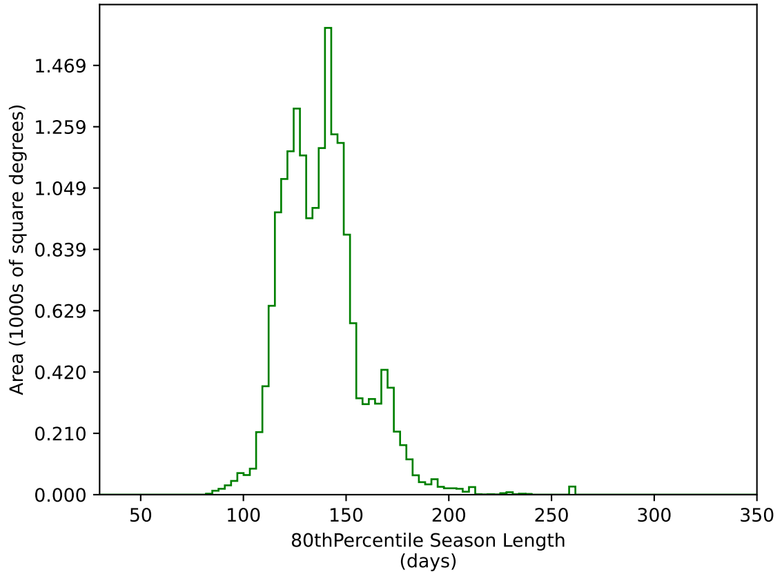
ddf_acor_sf10_lsf40_lsr10_v3.4_10yrs WFD g band: 80thPercentile Season Length
