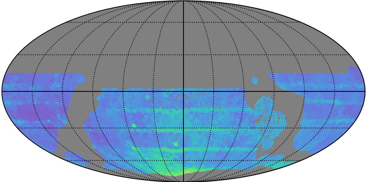
ddf_acor_sf10_lsf40_lsr10_v3.4_10yrs WFD all bands: 80thPercentile Season Length
