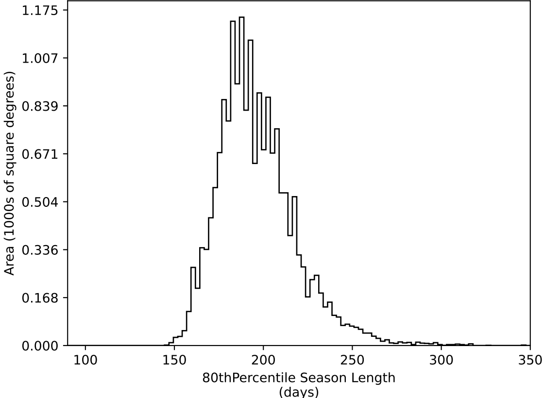
ddf_acor_sf10_lsf40_lsr10_v3.4_10yrs WFD all bands: 80thPercentile Season Length
