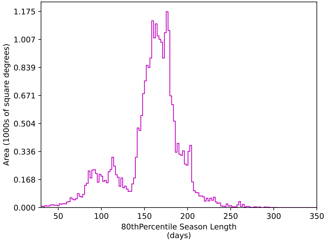
ddf_acor_sf10_lsf40_lsr10_v3.4_10yrs All sky z band: 80thPercentile Season Length
