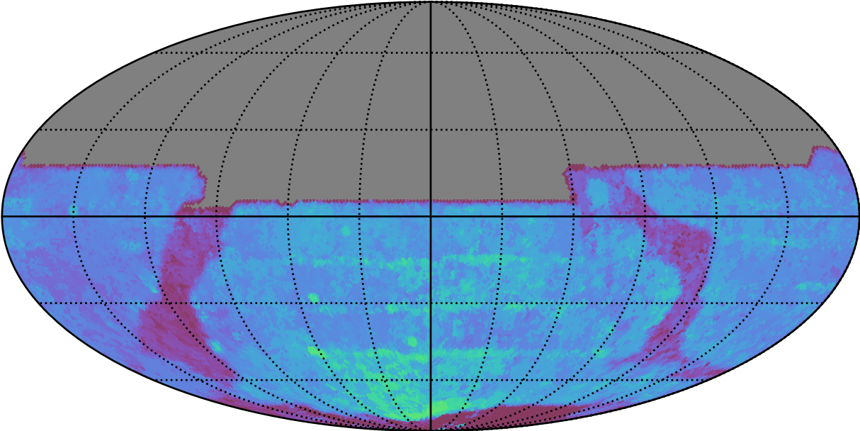
ddf_acor_sf10_lsf40_lsr10_v3.4_10yrs All sky y band: 80thPercentile Season Length
