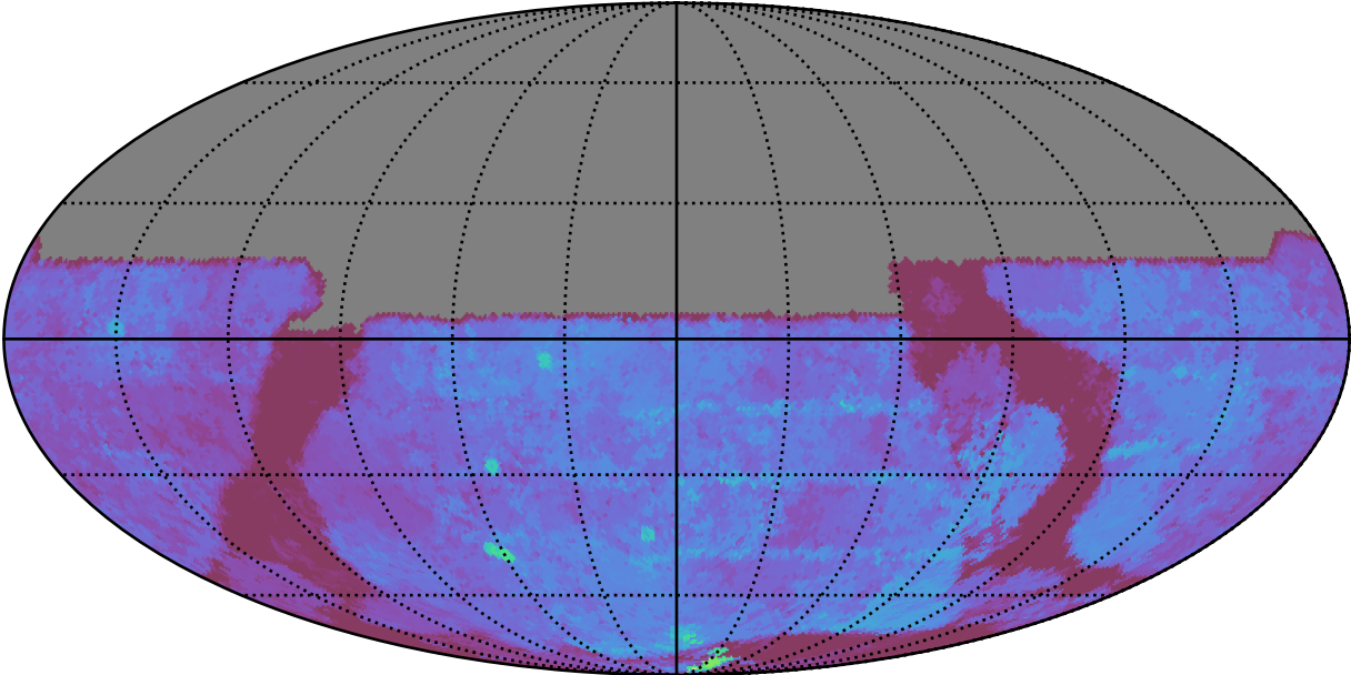
ddf_acor_sf10_lsf40_lsr10_v3.4_10yrs All sky u band: 80thPercentile Season Length
