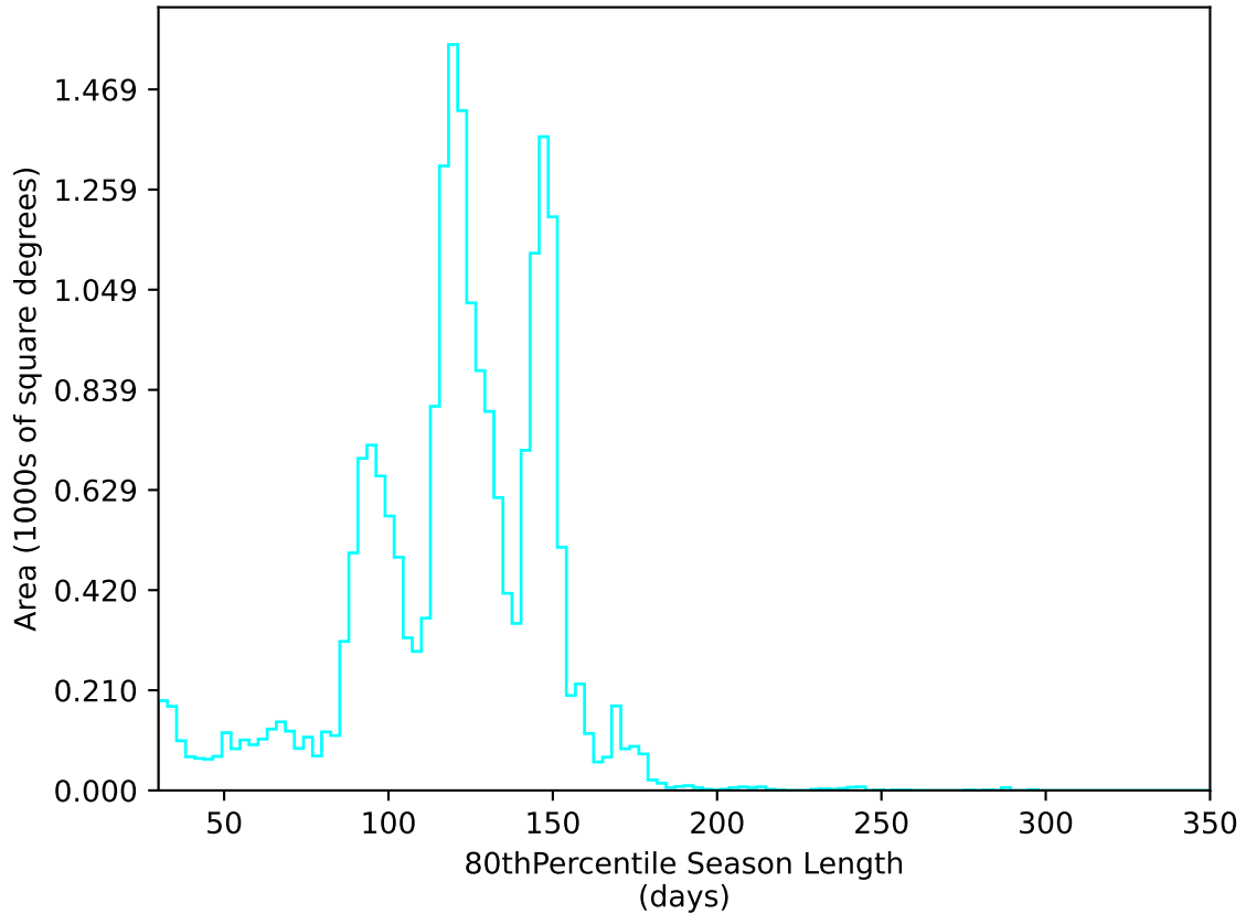
ddf_acor_sf10_lsf40_lsr10_v3.4_10yrs All sky u band: 80thPercentile Season Length
