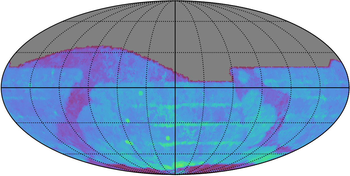
ddf_acor_sf10_lsf40_lsr10_v3.4_10yrs All sky r band: 80thPercentile Season Length
