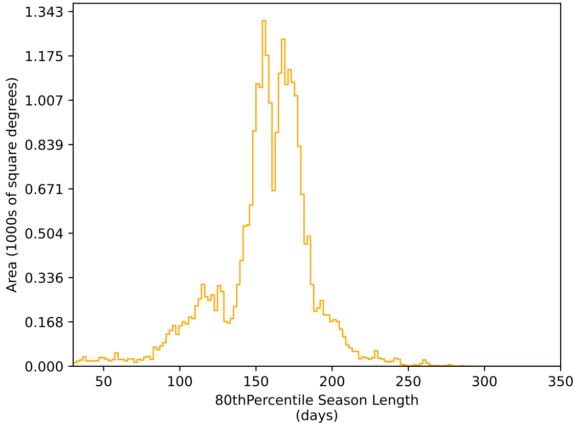
ddf_acor_sf10_lsf40_lsr10_v3.4_10yrs All sky r band: 80thPercentile Season Length
