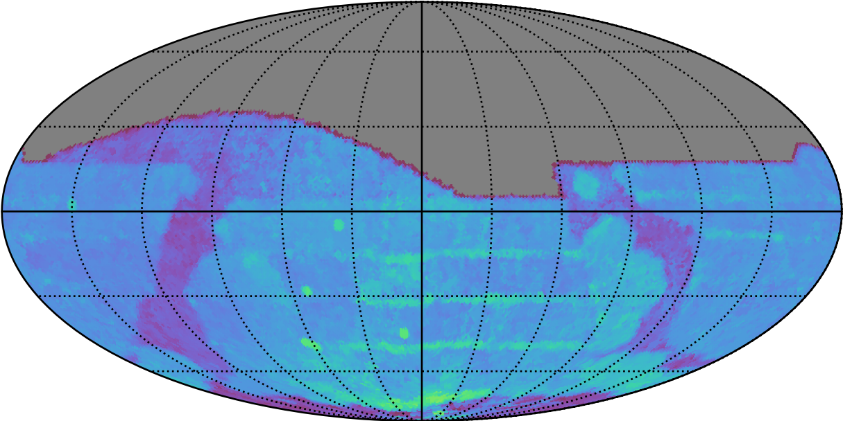
ddf_acor_sf10_lsf40_lsr10_v3.4_10yrs All sky i band: 80thPercentile Season Length
