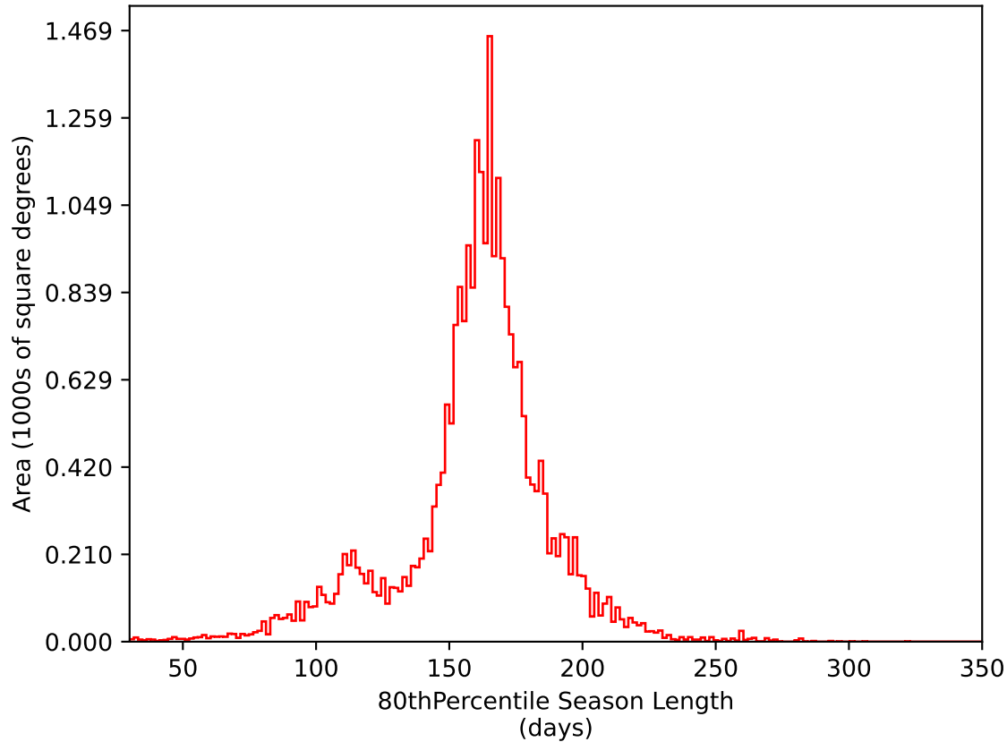
ddf_acor_sf10_lsf40_lsr10_v3.4_10yrs All sky i band: 80thPercentile Season Length
