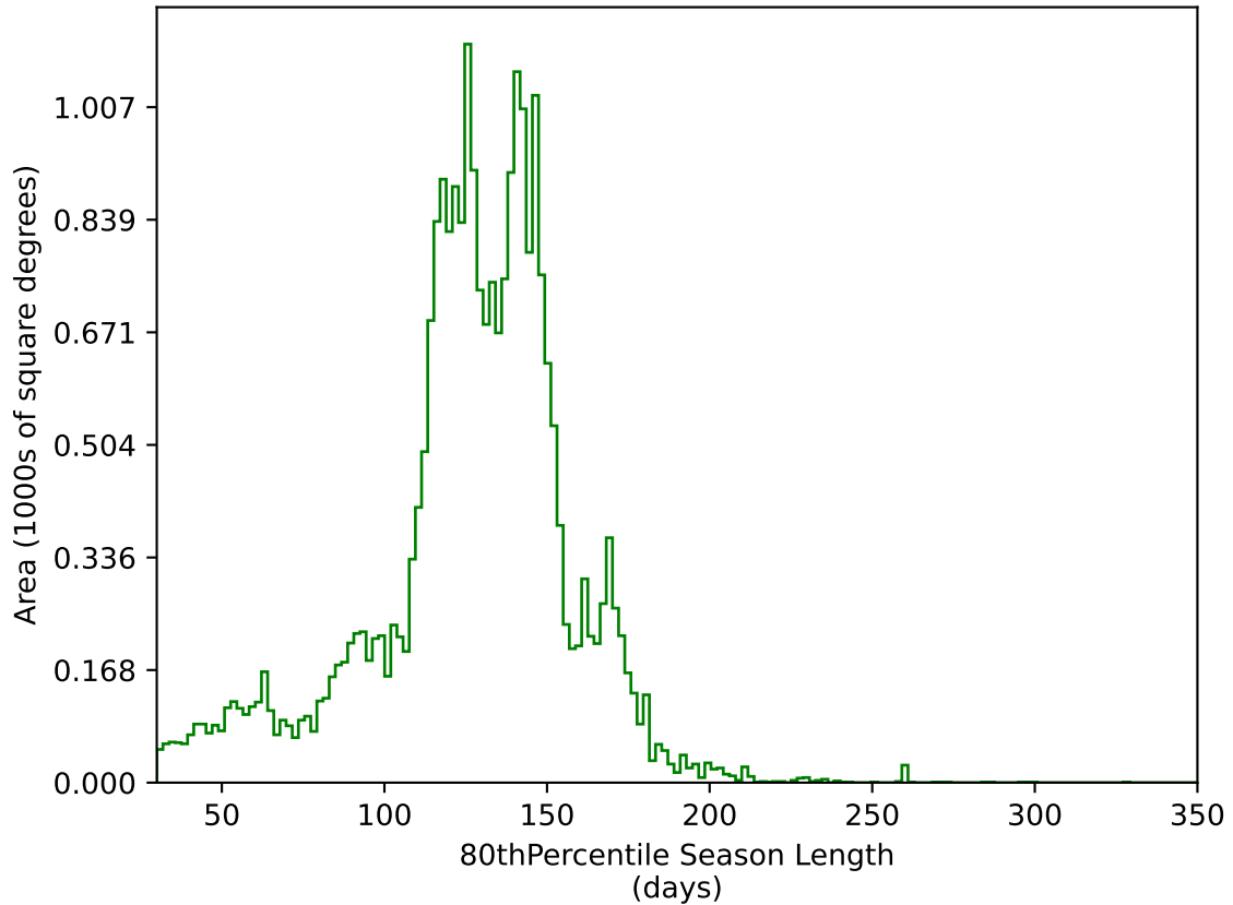
ddf_acor_sf10_lsf40_lsr10_v3.4_10yrs All sky g band: 80thPercentile Season Length
