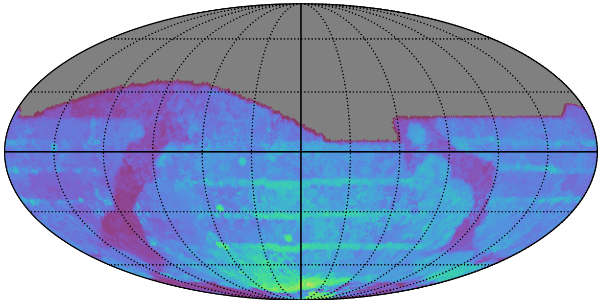
ddf_acor_sf10_lsf40_lsr10_v3.4_10yrs All sky all bands: 80thPercentile Season Length
