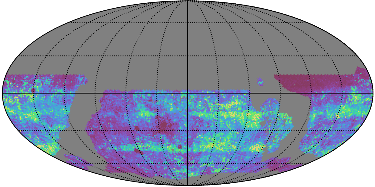
ddf_acor_sf10_lsf40_lsr10_v3.4_10yrs WFD zy bands: 75th Percentile Intranight Timespan
