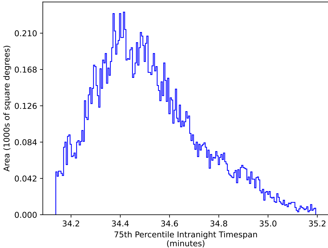
ddf_acor_sf10_lsf40_lsr10_v3.4_10yrs WFD zy bands: 75th Percentile Intranight Timespan
