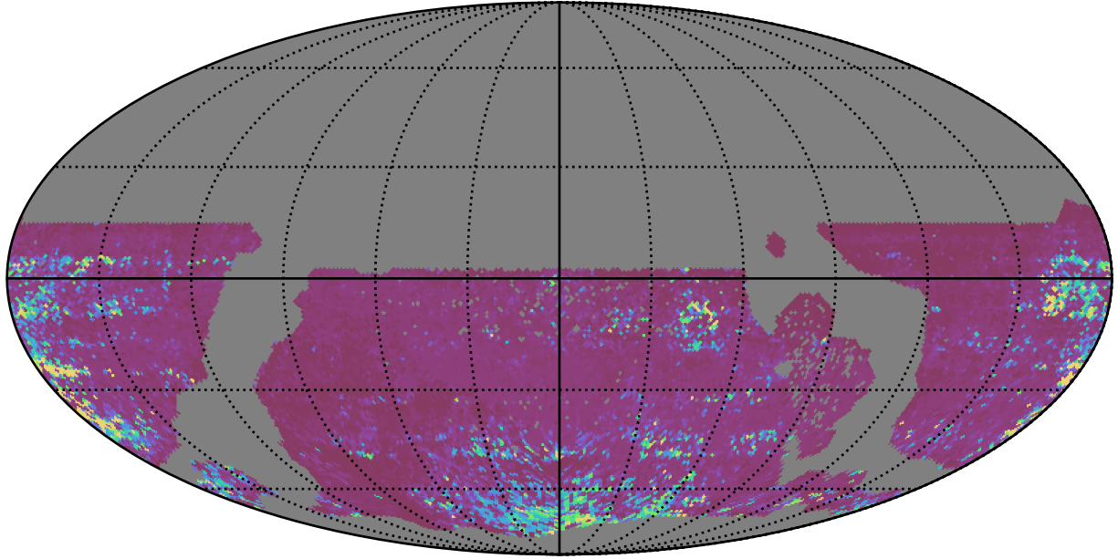
ddf_acor_sf10_lsf40_lsr10_v3.4_10yrs WFD z band: 75th Percentile Intranight Timespan
