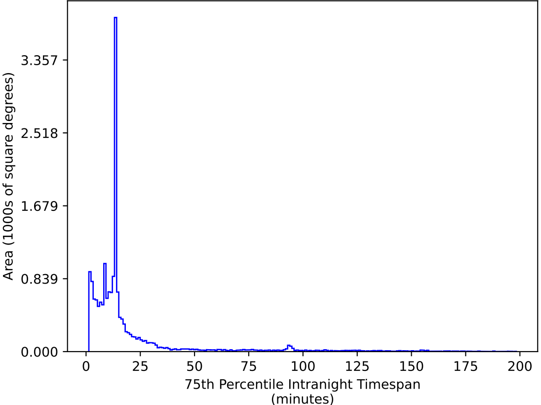
ddf_acor_sf10_lsf40_lsr10_v3.4_10yrs WFD z band: 75th Percentile Intranight Timespan
