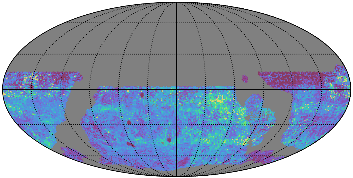
ddf_acor_sf10_lsr10_v3.4_10yrs WFD y band: 75th Percentile Intranight Timespan
