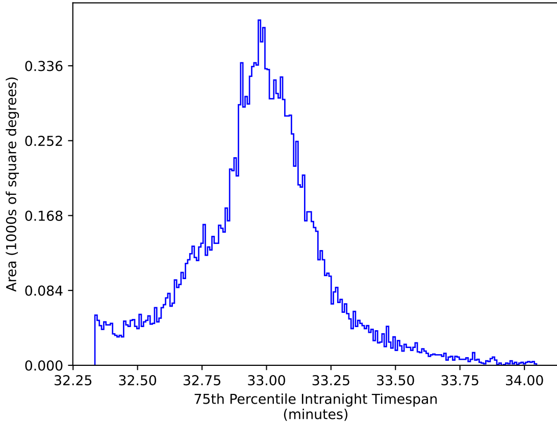
ddf_acor_sf10_lsf40_lsr10_v3.4_10yrs WFD y band: 75th Percentile Intranight Timespan
