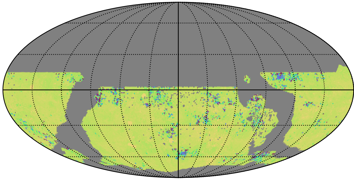
ddf_acor_sf10_lsf40_lsr10_v3.4_10yrs WFD ug bands: 75th Percentile Intranight Timespan
