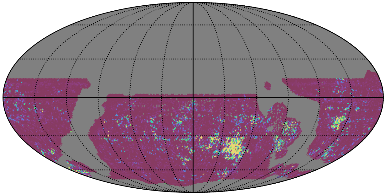
ddf_acor_sf10_lsf40_lsr10_v3.4_10yrs WFD u band: 75th Percentile Intranight Timespan
