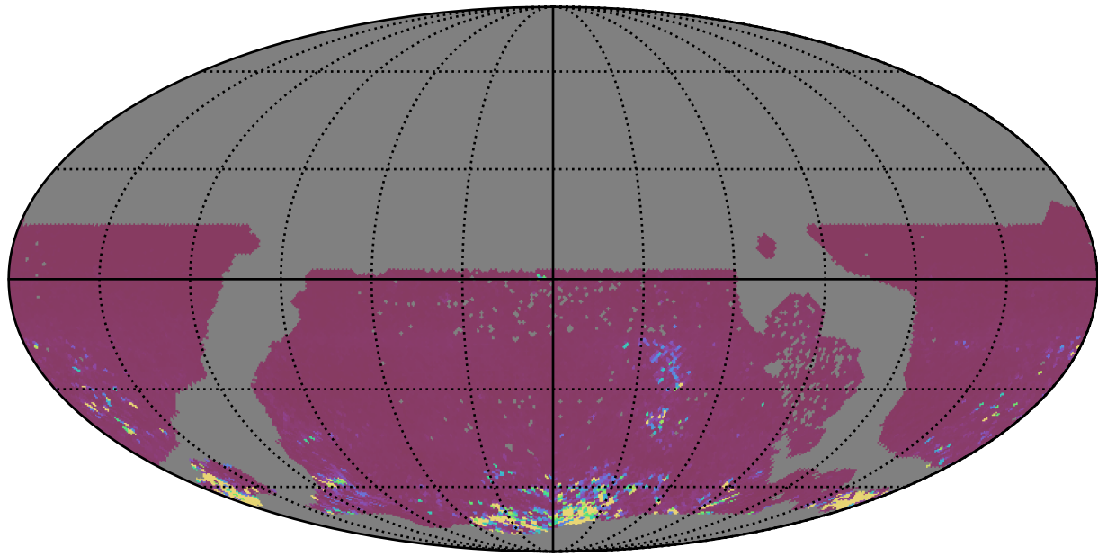
ddf_acor_sf10_lsf40_lsr10_v3.4_10yrs WFD ri bands: 75th Percentile Intranight Timespan
