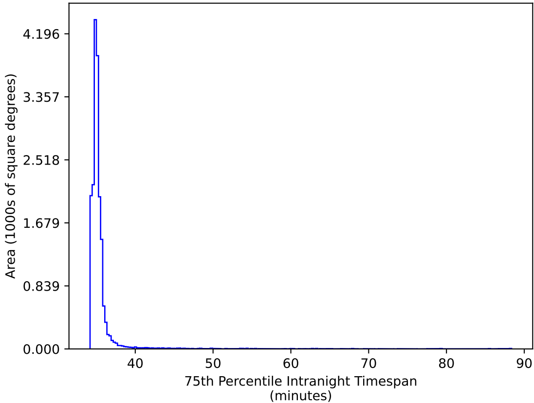
ddf_acor_sf10_lsf40_lsr10_v3.4_10yrs WFD ri bands: 75th Percentile Intranight Timespan
