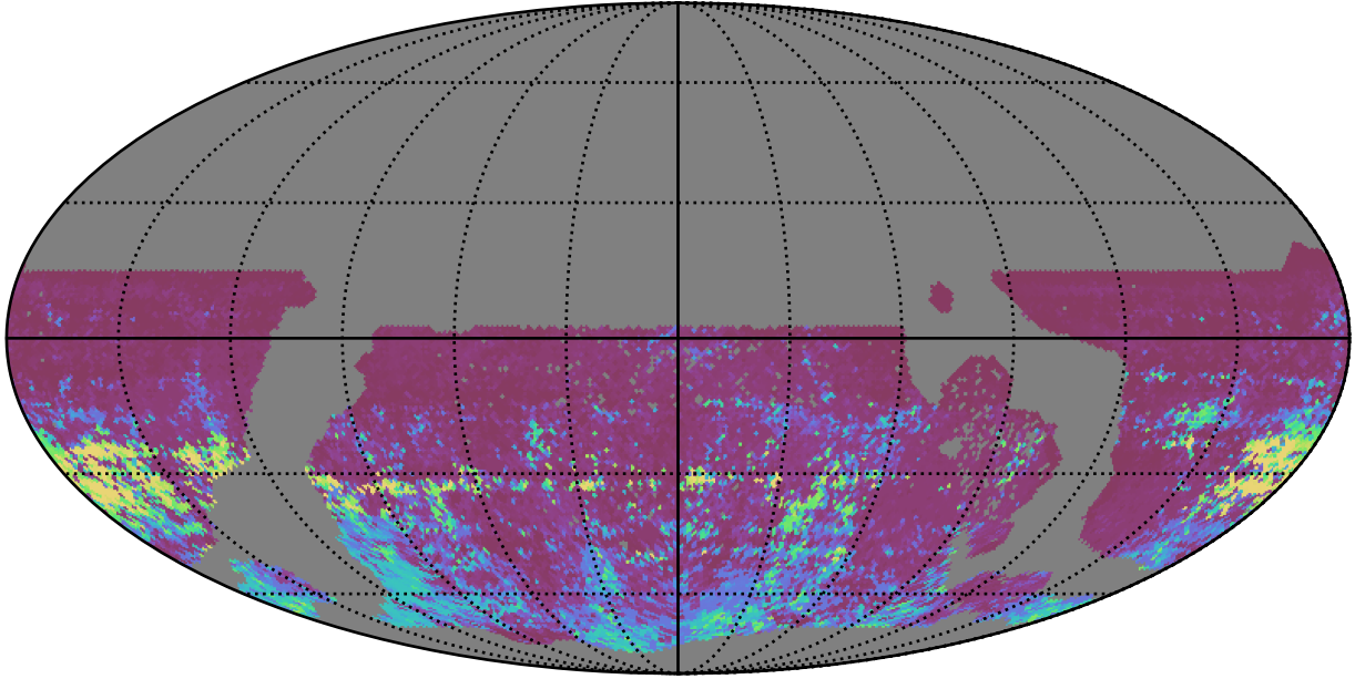
ddf_acor_sf10_lsf40_lsr10_v3.4_10yrs WFD r band: 75th Percentile Intranight Timespan
