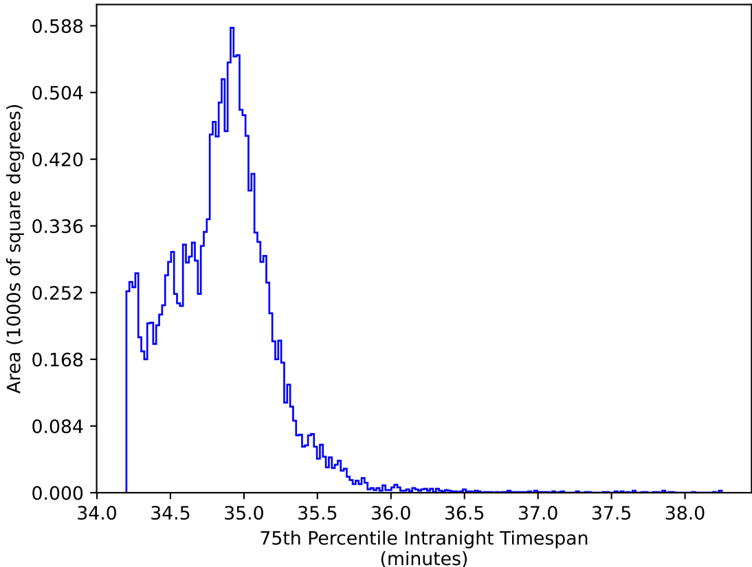
ddf_acor_sf10_ls40_lsr10_v3.4_10yrs WFD iz bands: 75th Percentile Intranight Timespan
